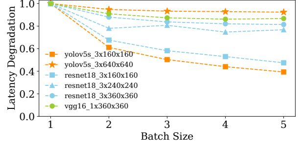
Figure 4: Batch Efficiency (evaluated under TensorRT on the edge platform NVIDIA Jetson TX2).
