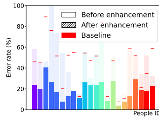
Fig. 30: In-the-wild evaluation per speaker.
