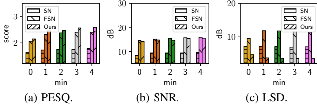
Fig. 15: Impact of calibration time.
