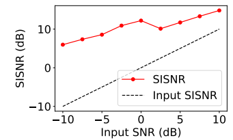
Fig. 27: Adaptive speech enhancement performance.
