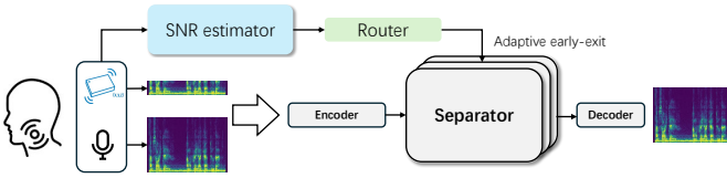
Fig. 14: Adaptive inference of VibOmni.
