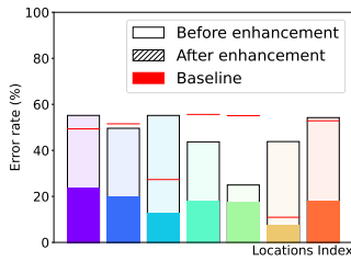
Fig. 29: In-the-wild evaluation per location.
