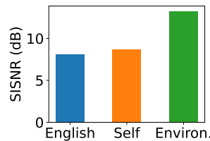
Fig. 5: Speech Enhancement on different kinds of noises.
