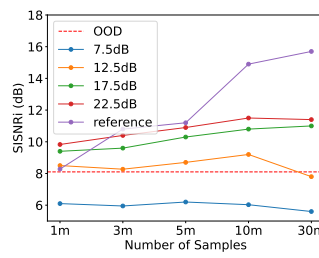
Fig. 25: Continual learning performance vs. SNR threshold
