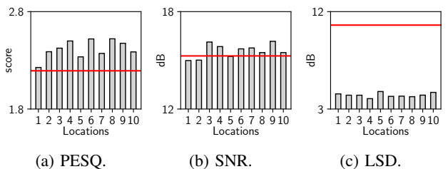
Fig. 20: VibVoice on different head locations. Red line: the performance of the baseline, i.e., FullSubNet.
