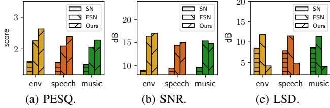
Fig. 16: Impact of noise types.
