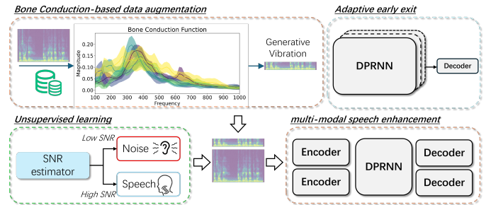
Fig. 8: Overview of the VibOmni pipeline, including multi-modal enhancement, BCF-based pre-training, continual learning, and adaptive inference.
