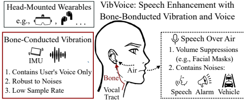
Fig. 1: VibOmni enhances speech quality of head-mounted wearables by extracting the user's clear voice from the bone-conducted vibrations.
