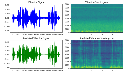
Fig. 12: Vibration and the reconstructed vibration.
