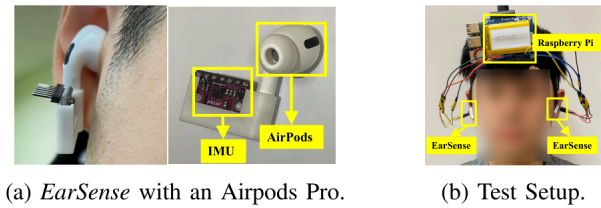
Fig. 2: EarSense is an open-sourced data collector attachable to commercial earables for vibration sensing.
