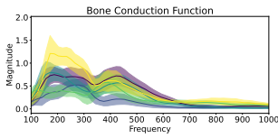
Fig. 10: BCF of dataset 1.
