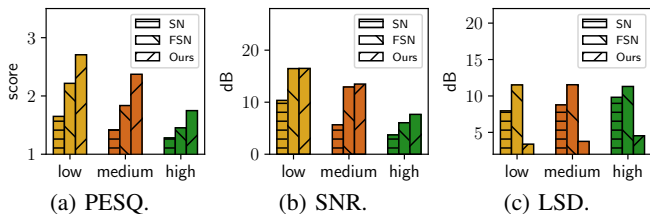
Fig. 17: Impact of noise levels.
